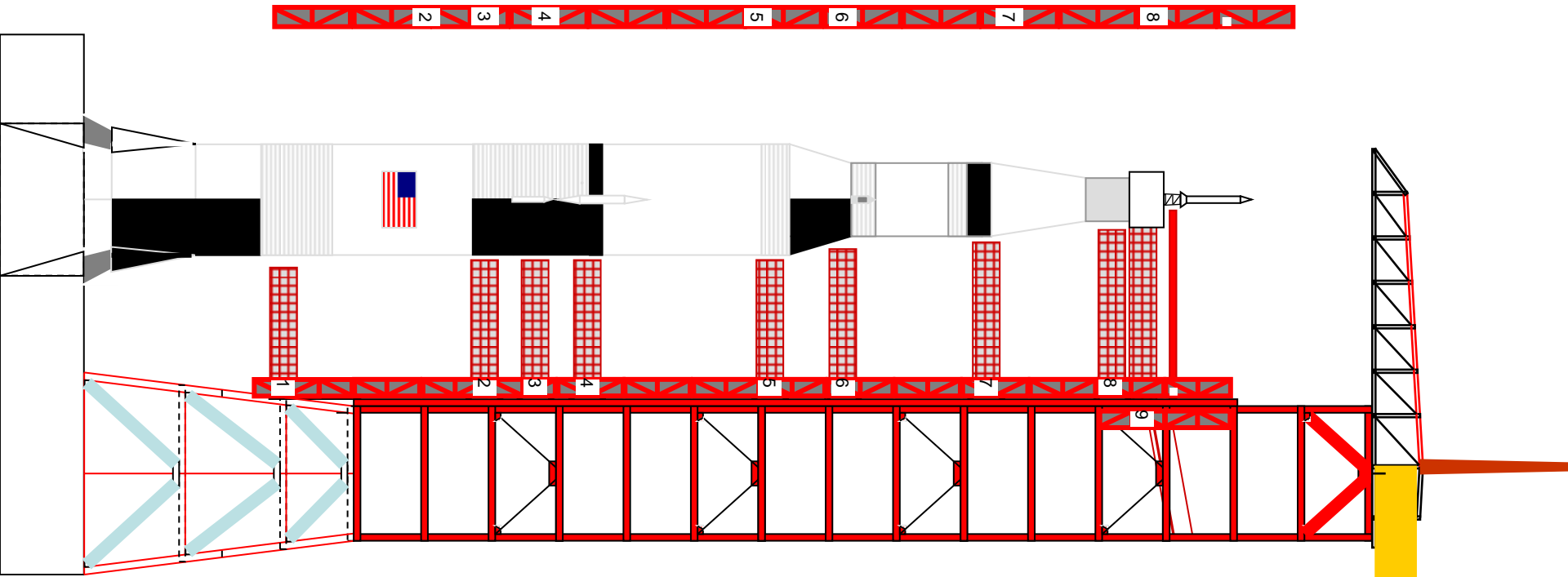
Access Arm Girder, Base Section – Side 1
